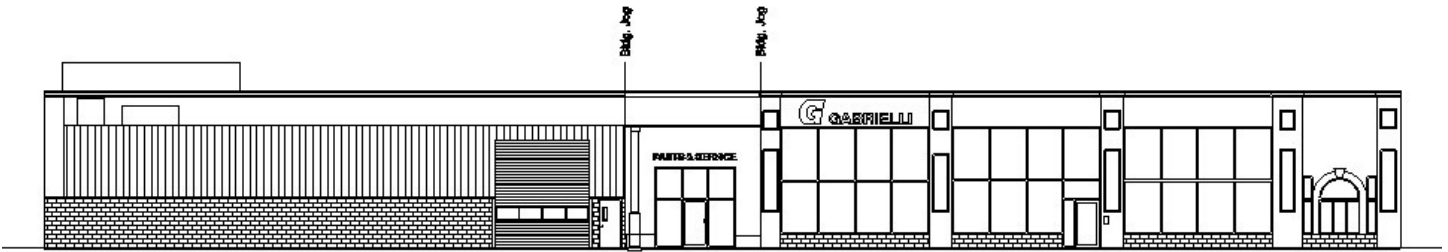
48 Bridgeville Road Front Elevation
