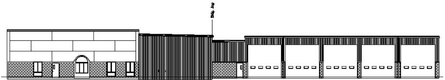
48 Bridgeville Road Right Side Elevation
