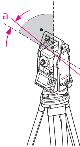
Tilting-axis error (a)
