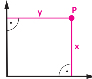
Cartesian coordinates
